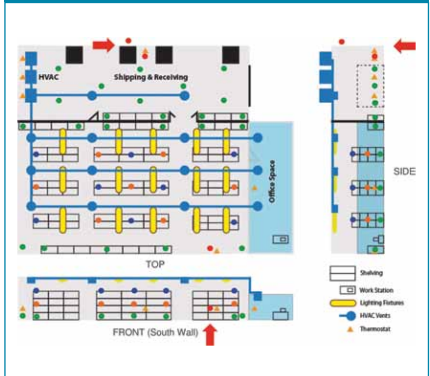
Figure 11: Sensor placement sample; sensors are green, blue and orange dots at different heights.
